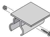
Standing-seam clamp
