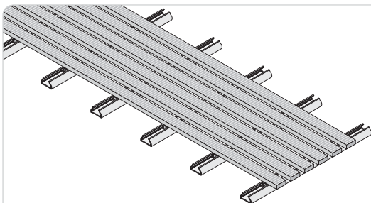
Longways system for single-ply membrane roofing
